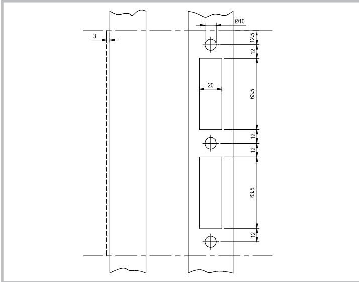
Lock case 5018/5032: aluminium frame
