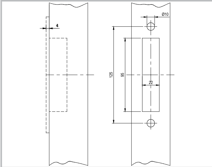
Lock case 5049: aluminium frame
