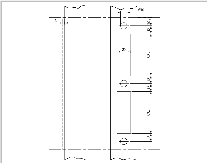
Lock case 5016: aluminium frame
