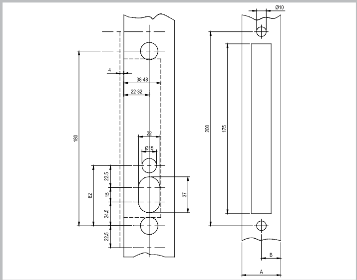
Lock case 5049: aluminium door
