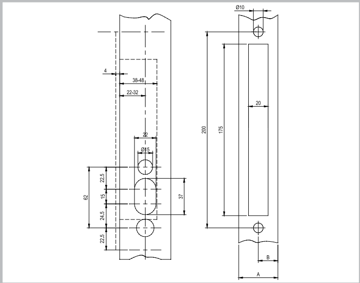
Lock case 5018/5032: aluminium door
