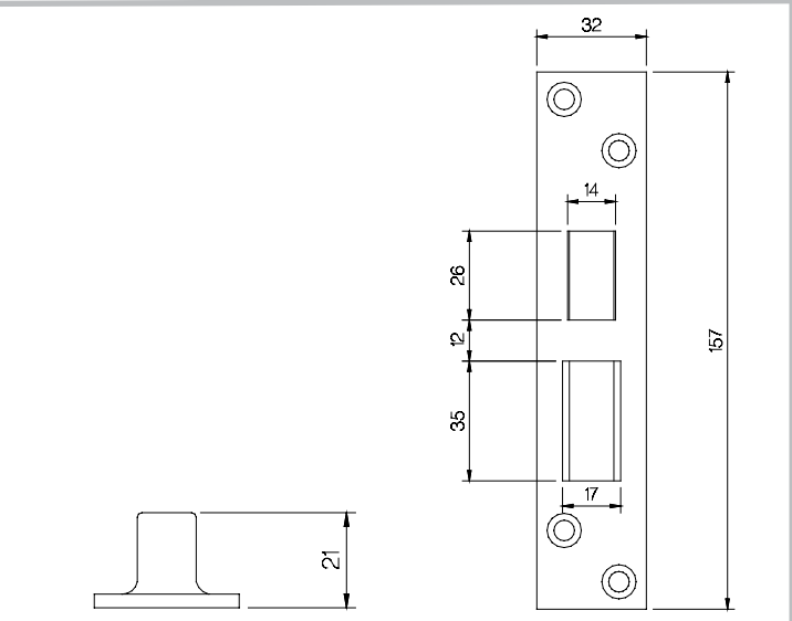
Striker plate for 5382/8 only (supplied with or without dust box)
