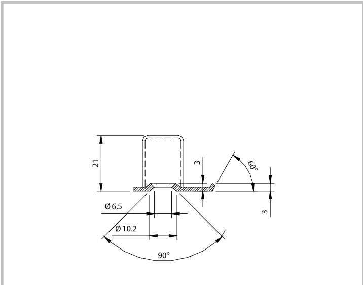
Striker plate with dust box for 53-Series
