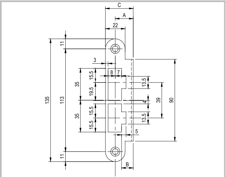
Striker plate for 5320/8 only
