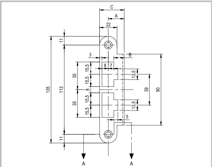
Striker plate for 53-Series (excluding 5320/8 and 5382/8)
