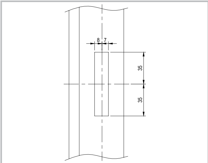
Striker plate cut out
